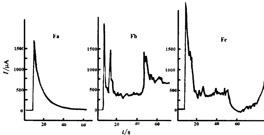
图4 不同的载荷条件下18/8 不锈钢在2 mmol/L Na_2S_2O_3 + 0.1% HCl 溶液中恒电位为0.0 V(SEC)时暂态极化电流的测量 Fig. 4 Polarization current transients of 18/8 stainless steel in 2 mmol/L Na_2S_2O_3 + 0.1% HCl solution at 0.0 V(SEC) under the different loading condition, F_a < F_b < F_c
