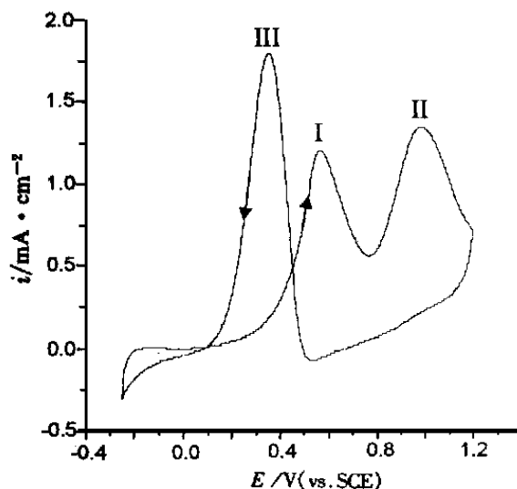
图 1 乙醇在 nm-Pt/GC 电极上氧化的循环伏安曲线 Fig. 1 Cyclic Voltammogram of \text{CH}_3\text{CH}_2\text{OH} Oxidation on nm-Pt/GC electrode in 0.1 \text{ mol} \cdot \text{L}^{-1} \text{H}_2\text{SO}_4 + 0.1 \text{ mol} \cdot \text{L}^{-1} \text{CH}_3\text{CH}_2\text{OH} solution, sweep rate: 50 \text{ mV} \cdot \text{s}^{-1}
