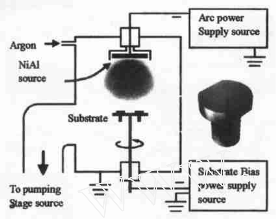
图 1 阴极电弧放电被覆设备示意图及试片外观 图 2 坑蚀试验设备示意图 Fig. 1 Schematic diagram of a cathodic arc plasma ion plating system and the specimen geometry Fig. 2 Cavitation test experimental setup
