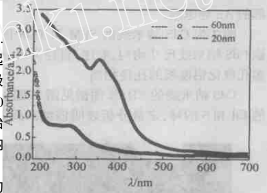
图 5 不同尺寸的 CdS 纳米线阵列的吸收光谱 Fig.5 UV-Vis absorption spectrum of the CdS nanowire arrays with different diameters
