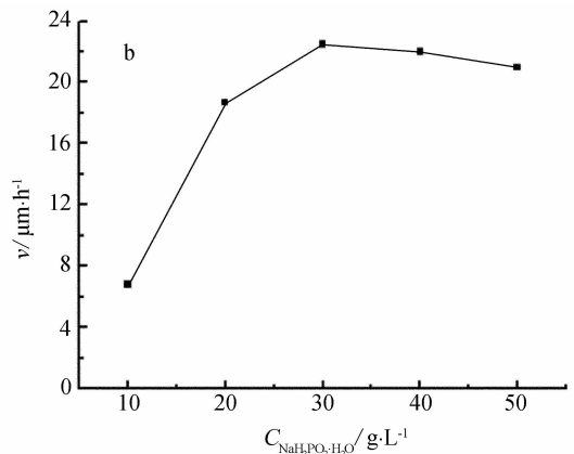
Fig. 3 Effects of nickel sulfate(a) and sodium hypophosphite(b) contents in bath on the electroless nickel deposition rate
