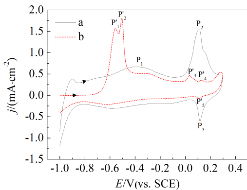
图 2 CoPt/GC 电极饱和和吸附 CO 前(a)、后(b)0.1 mol·L -1 NaOH 溶液中的循环伏安曲线, 扫描速率: 50 mV·s -1 Fig. 2 Cyclic voltammograms of CoPt/GC electrode before (a) and after (b) saturated with CO in 0.1 mol·L -1 NaOH solution, scan rate: 50 mV·s -1
