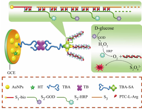
图 8 双酶催化产生溶解氧的适体传感器制备示意图 [33] Fig. 8 Schematic diagram showing the dual signal amplification strategy for ECL detection of TB [33]
