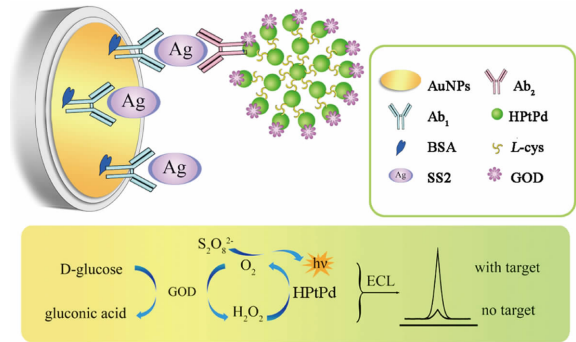
图 9 GOD 和 HPTd 仿双酶免疫传感器制备及催化机理示意图 [37] Fig. 9 Schematic diagram of preparation and reaction mechanism of the ECL immunosensor [37]
