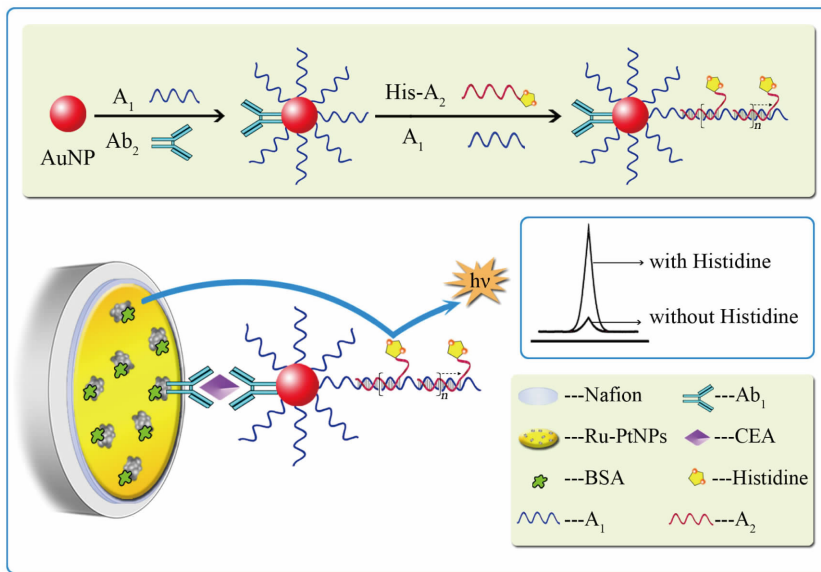
图 5 超夹心 DNA 放大技术的免疫传感器制备及放大原理示意图 [24] Fig. 5 The schematic diagrams of the immunosensor and signal amplification mechanism [24]
