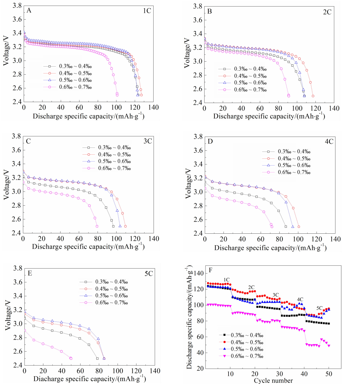
图 2 不同水分含量电池在 1C ~ 5C 倍率下的放电曲线(A-E)以及不同水分含量电池的倍率性能对比(F) Fig. 2 Rate discharge curves of LFP/1C (A), LFP/2C (B), LFP/3C (C), LFP/4C (D), LFP/5C (E), and comparison of rate capability of LFP lithium-ion battery with different water contents (F)
