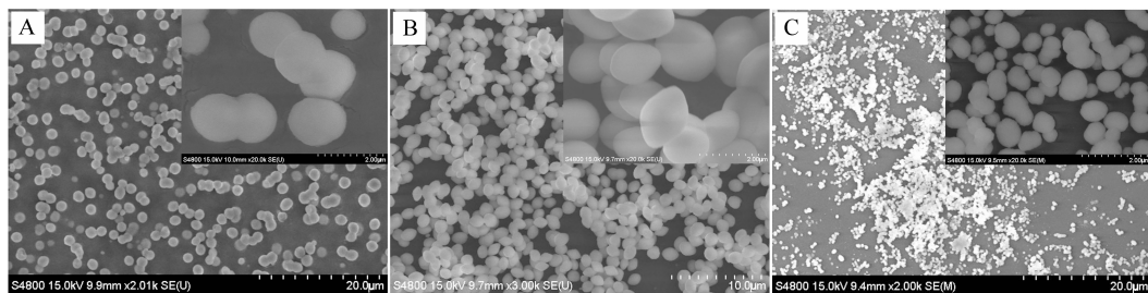
图 4 不同温度下制备样品的 SEM 照片(插图为高放大倍率电镜图片) A. 60 °C; B. 80 °C; C. 100 °C Fig. 4 SEM images of the samples prepared at different temperatures (the insets are high magnification images) A. 60 °C; B. 80 °C; C. 100 °C
