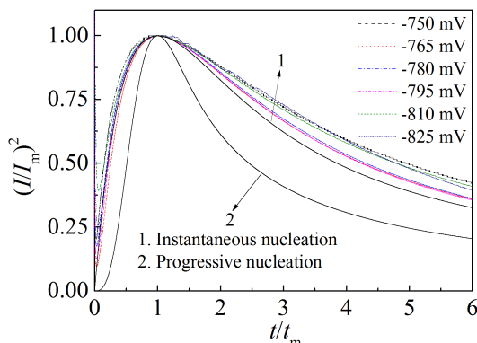
图 3 不同施加电位下实验曲线与理论曲线对比图 Fig. 3 Comparisons between experimental curves and theoretical curves at different potentials
