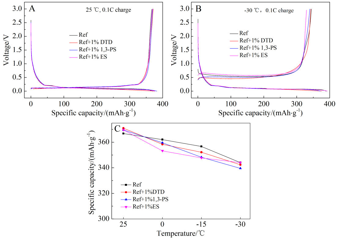
图 4 AG/Li 半电池在不同电解液中的 25 °C 下充放电曲线(A)、25 °C 放电、-30 °C 下充电的曲线(B)及不同温度下的充电容量(C) Fig. 4 The electrochemical data of AG/Li half cells with different electrolytes. (A) charged/discharged at 25 °C; (B) discharged at 25 °C, charged at -30 °C and (C) temperature dependent charge capacity
