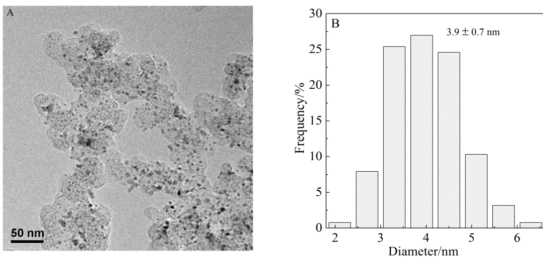
Fig. S1 (A) TEM image of Pd/C and (B) the corresponding histograms of particle size
