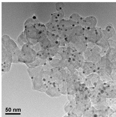
Fig. S3 TEM image of the as-prepared Au@Pd (120 s) NPs
