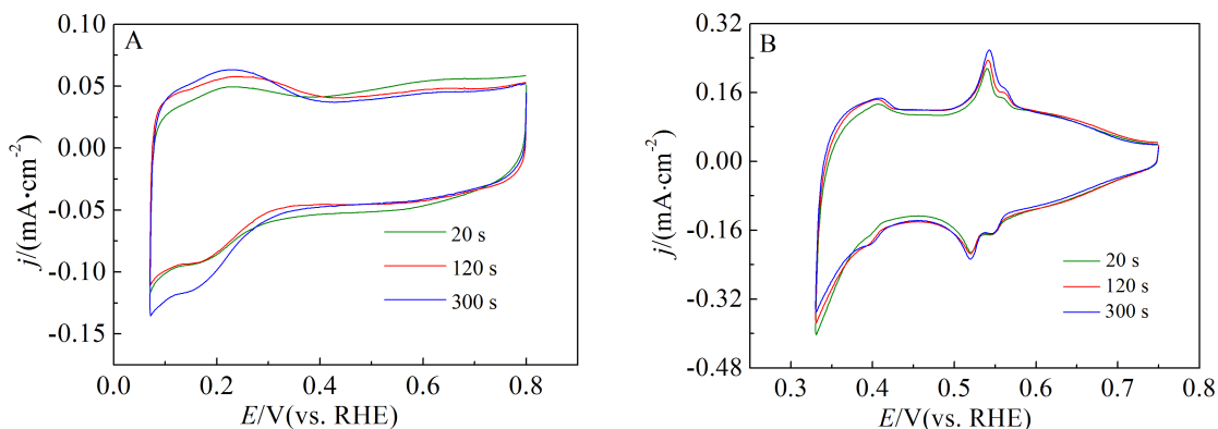
Fig. S2 Cyclic voltammograms of Au@Pd/C (20 s, 120 s and 300 s) electrodes in a deaerated (A) 0.1 mol·L -1 HClO 4 solution and (B) 0.05 mol·L -1 H 2 SO 4 + 0.05 mol·L -1 CuSO 4 solution. Scanning rate = 50 mV·s -1 . The currents were normalized to the geometric area of the electrode (0.196 cm 2 ).
