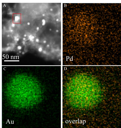
Fig. S5 (A) an HAADF-STEM image of the as-prepared Au@Pd (300 s) NPs and (B-D) the corresponding EDX elemental 2D mapping images of Pd (orange), Au (green) and overlap.
