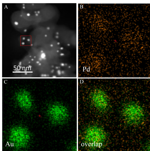
Fig. S4 (A) an HAADF-STEM image of Au@Pd/C (20 s) and (B-D) the corresponding EDX elemental 2D mapping images of Pd (orange), Au (green) and overlap.
