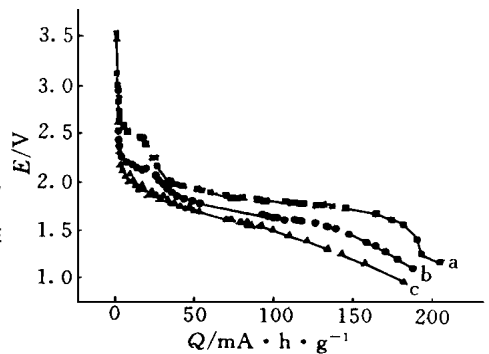
图 1 \text{Li} | 1 \text{ mol/L LiClO}_4 + \text{PC} + \text{DME} | \alpha\text{-Sn}(\text{HPO}_4)_2 乙炔黑电池的放电曲线, 25 °C a) 15 \mu\text{A}/\text{cm}^2 ; b) 50 \mu\text{A}/\text{cm}^2 ; c) 80 \mu\text{A}/\text{cm}^2
