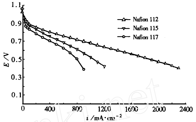
图3 质子交换膜厚度不同时 PEMFC 的电压~电流密度变化曲线 Fig. 3 Cell potential vs. current density plots for PEMFC containing Nafion 117, Nafion 115 and Nafion 112. T_{\text{cell}} = 80 , T_{\text{H}_2} = T_{\text{O}_2} = 90 , P_{\text{H}_2} = 0.3 \text{ MPa} , P_{\text{O}_2} = 0.5 \text{ MPa}
