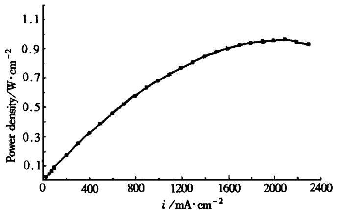
图4 Nafion 112 膜和 E-TEK 电极组装的 PEMFC 功率密度与电流密度变化曲线 Fig. 4 Cell power density vs. current density plot for PEMFC using Nafion 112 and E-TEK electrode. The operation conditions of cell is the same as those of Fig. 3
