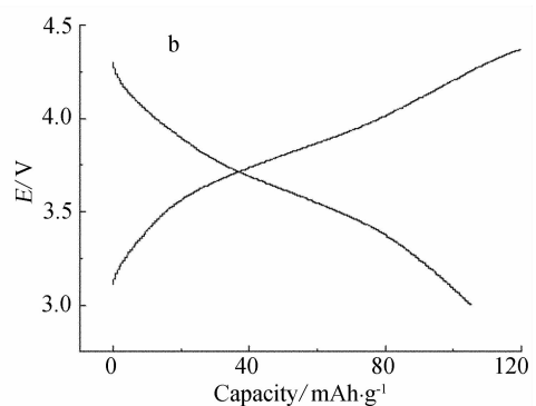
图 4 PTPAn(a) 及 PTPAn/活性炭电极(b) 0.5\text{C} 的充放电曲线 Fig. 4 Charge and discharge curves of the as-prepared PTPAn (a) and PTPAn/active carbon compound (b) at 0.5\text{ C} rate
