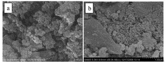
图 3 PTPAn(a) 及 PTPAn/活性炭复合材料(b) 的扫描电镜照片 Fig. 3 SEM image of the as-prepared PTPAn (a) and PTPAn/active carbon compound (b)
