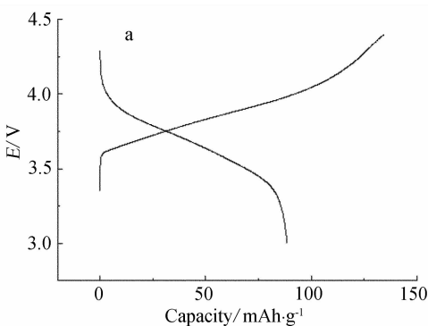
图 4 PTPAn(a) 及 PTPAn/活性炭电极(b) 0.5\text{C} 的充放电曲线 Fig. 4 Charge and discharge curves of the as-prepared PTPAn (a) and PTPAn/active carbon compound (b) at 0.5\text{ C} rate
