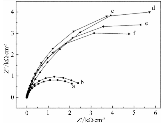
图 2 316L 钢在含有不同浓度 SDDTC 的原油模拟液 (pH=4,12 h) 中的阻抗曲线 Fig. 2 Impedance curves of the 316L steel in the crude simulation solution containing different concentrations of SDDTC C_{\text{SDDTC}}/\text{g} \cdot \text{L}^{-1} : a. 0; b. 0.38; c. 0.76; d. 1.14; e. 1.52; f. 1.9, scan rate: 5 \text{ mV} \cdot \text{s}^{-1} , pH=4, 12 h
