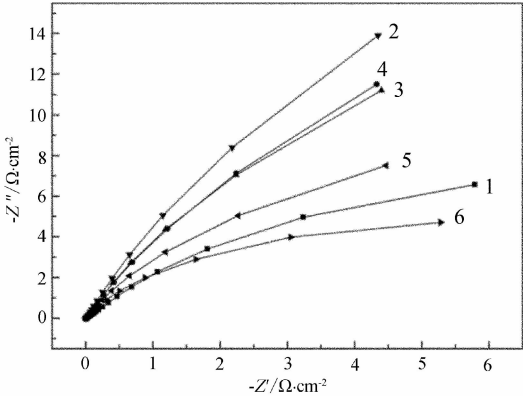
图 7 316L 钢在含有不同配比的 SDDTC-铬酸钠复配缓蚀剂的原油模拟液中的阻抗曲线 Fig. 7 Impedance curves of the 316L steel in the crude simulation solution containing different combinations of SDDTC compound with sodium chromate C_{\text{SDDTC}}/\text{g} \cdot \text{L}^{-1} + C_{\text{Na}_2\text{CrO}_4}/\text{g} \cdot \text{L}^{-1} : 1. 0.76 + 0.05; 2. 0.76 + 0.1; 3. 0.76 + 0.15; 4. 1.14 + 0.05; 5. 1.14 + 0.1; 6. 1.14 + 0.15
