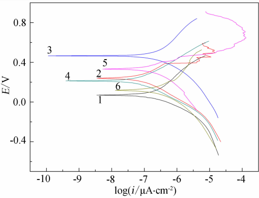
图 6 316L 钢在含有不同配比的 SDDTC-铬酸钠复配缓蚀剂原油模拟液中的极化曲线 Fig. 6 Polarization curves of the 316L steel in the crude simulation solution containing different combinations of SDDTC compound with sodium chromate C_{\text{SDDTC}}/\text{g} \cdot \text{L}^{-1} + C_{\text{Na}_2\text{CrO}_4}/\text{g} \cdot \text{L}^{-1} : 1. 0.76 + 0.05; 2. 0.76 + 0.1; 3. 0.76 + 0.15; 4. 1.14 + 0.05; 5. 1.14 + 0.1; 6. 1.14 + 0.15
