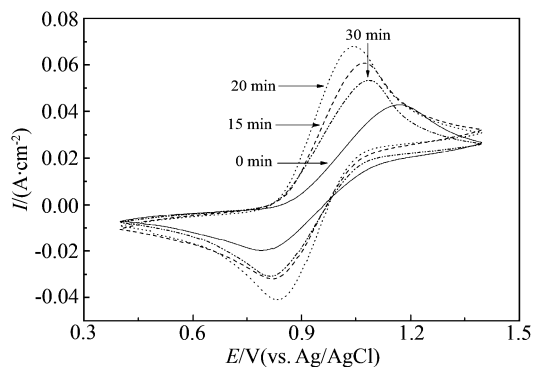
图 5 不同氧气等离子体处理时间的石墨电极在 2 \text{mol}\cdot\text{L}^{-1} \text{VOSO}_4 + 2 \text{mol}\cdot\text{L}^{-1} \text{H}_2\text{SO}_4 溶液中的循环伏安曲线(扫速 10 \text{mV}\cdot\text{s}^{-1} ) Fig. 5 CV curves of untreated and oxygen plasma treated graphite plate electrodes for different time, recorded at 10 \text{mV}\cdot\text{s}^{-1} in 2 \text{mol}\cdot\text{L}^{-1} \text{VOSO}_4 + 2 \text{mol}\cdot\text{L}^{-1} \text{H}_2\text{SO}_4 solution
